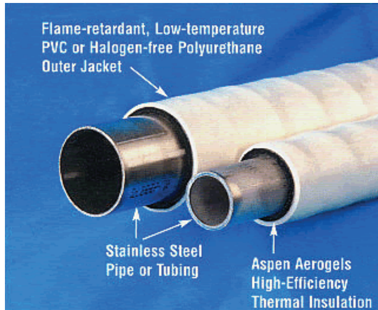
Dekoron/Unitherm BPE-6200 Preinsulated Pipe
